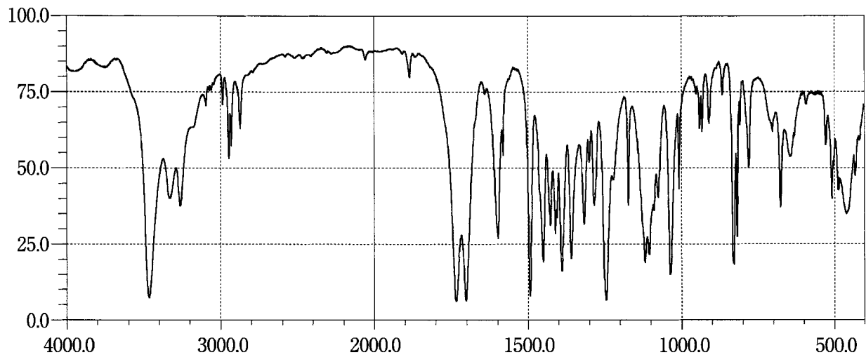
Chlorphenesin Carbamate
