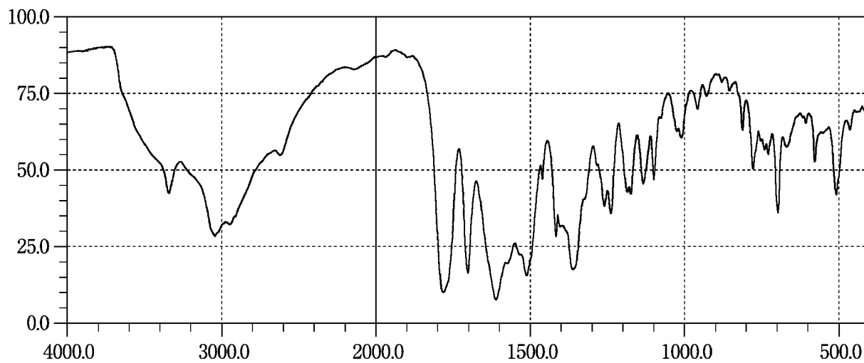
Cefaclor
