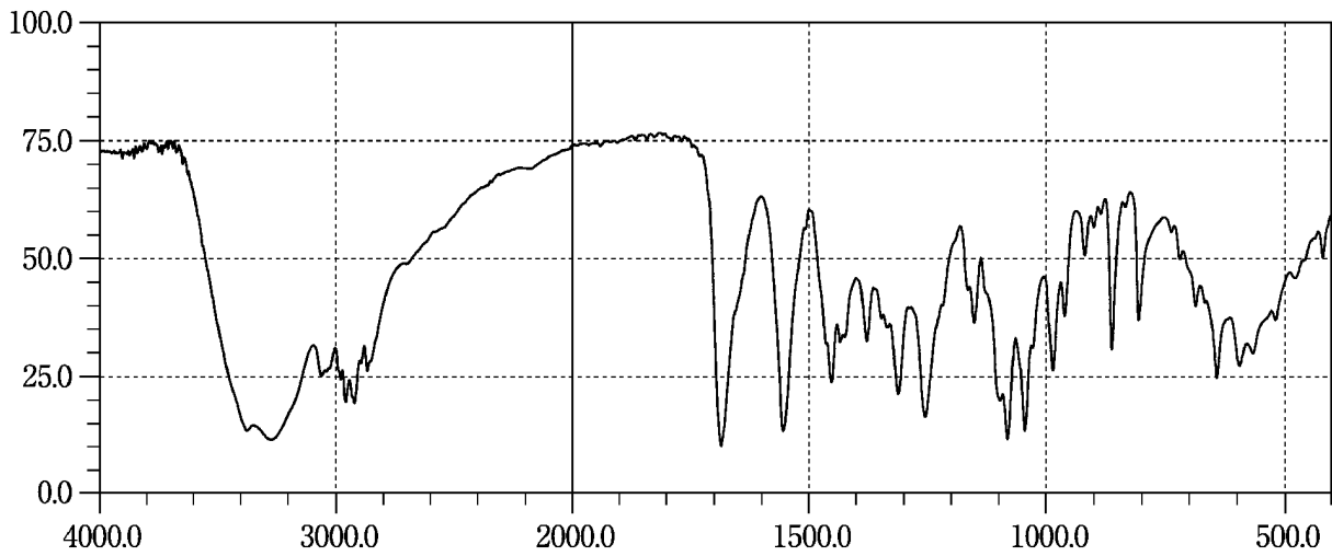
Clindamycin Hydrochloride
