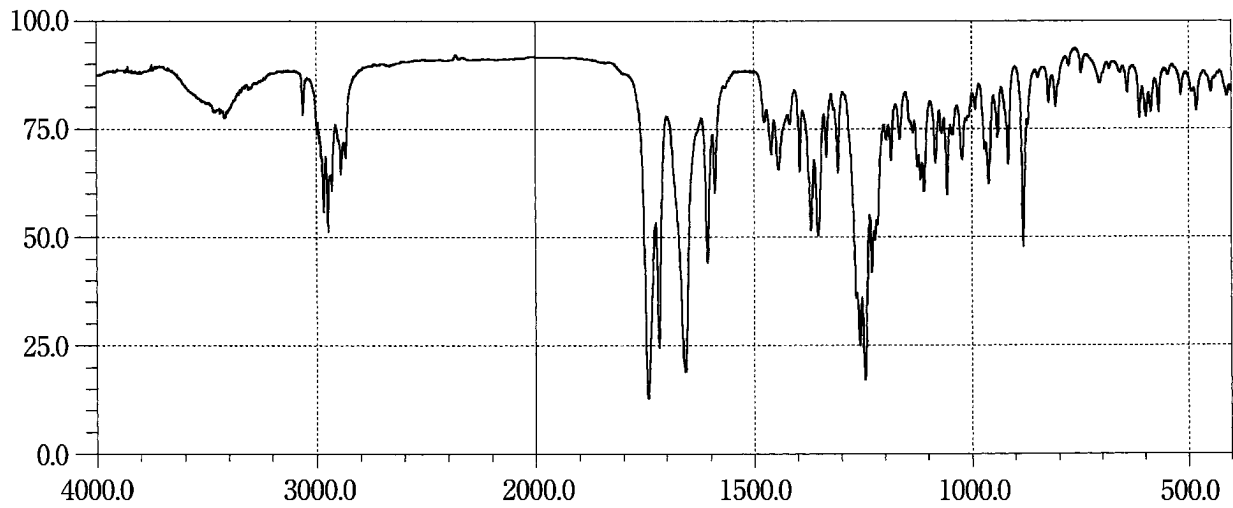
Chlormadinone Acetate
