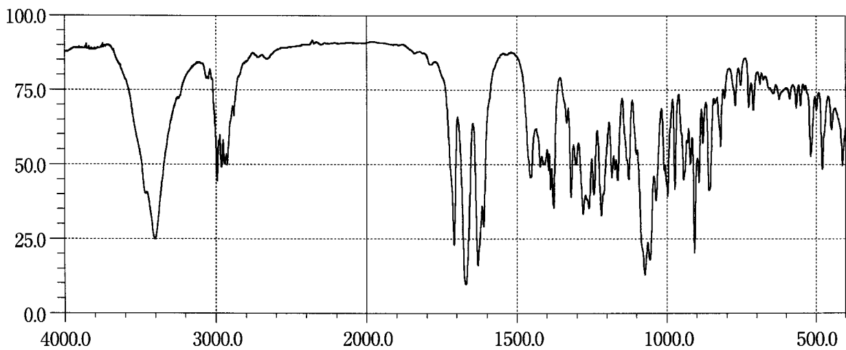
Fluocinolone Acetonide
