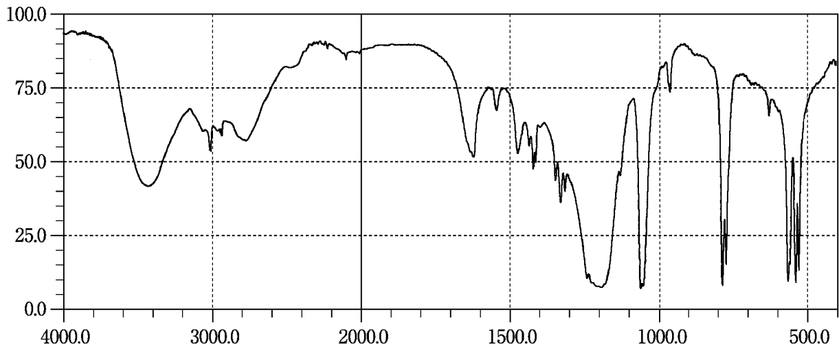
Betahistine Mesilate
