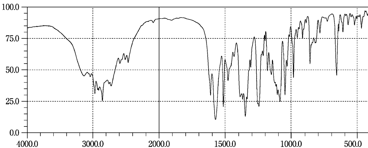
Bisoprolol Fumarate
