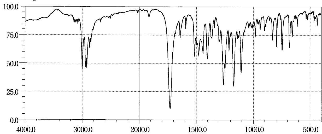
Distigmine Bromide
