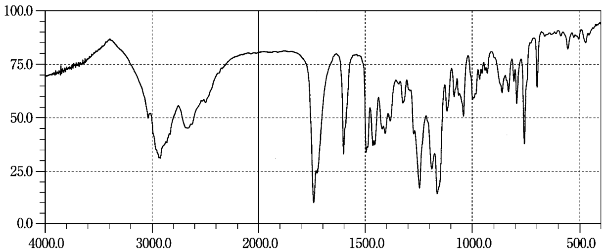
Sarpogrelate Hydrochloride
