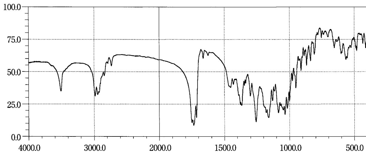
Midecamycin Acetate
