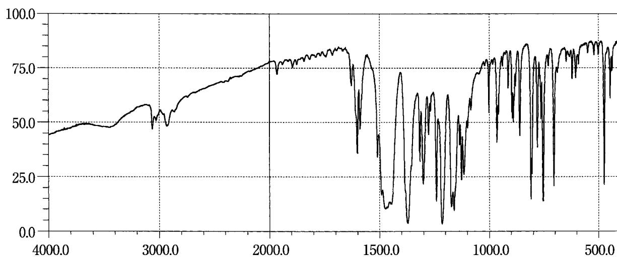
Tolnaftate
