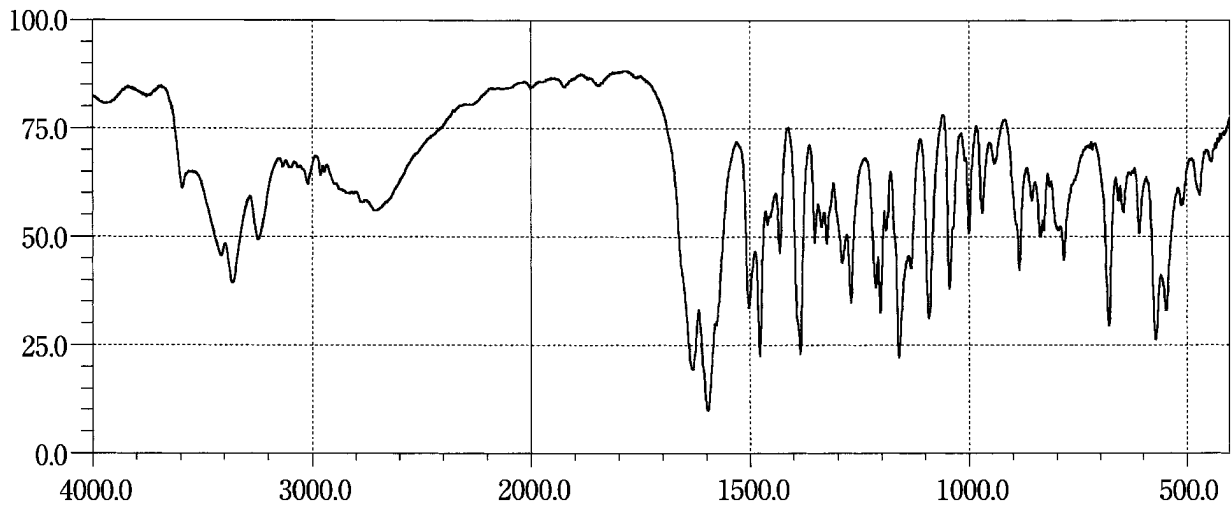
Sulfamonomethoxine Hydrate
