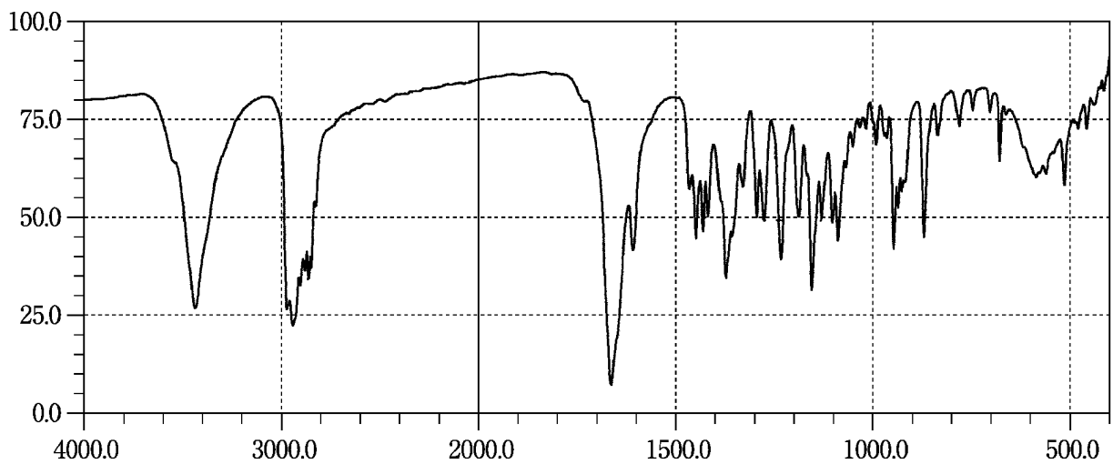
Methyltestosterone
