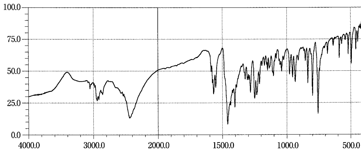
Thioridazine Hydrochloride
