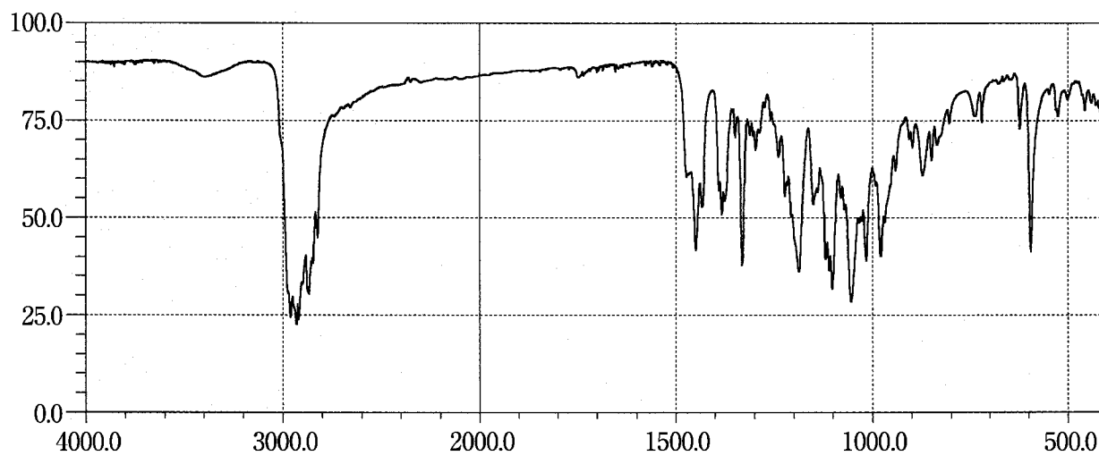
Mepitiostane
