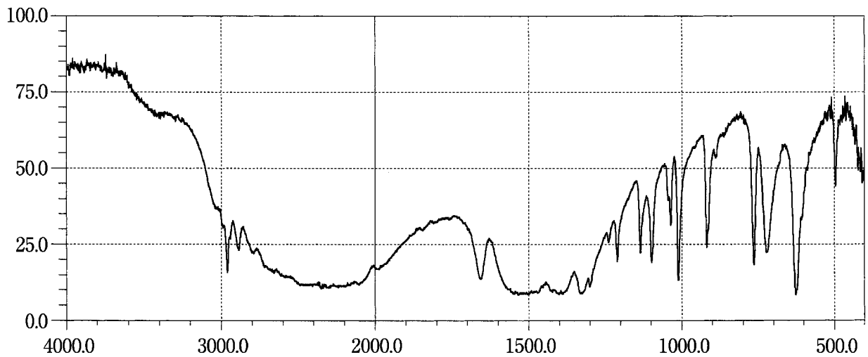
Piperazine Adipate
