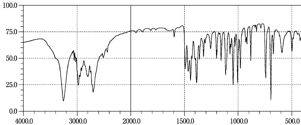
dl-Methylephedrine Hydrochloride
