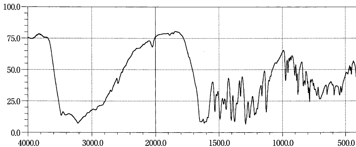
Methyldopa Hydrate
