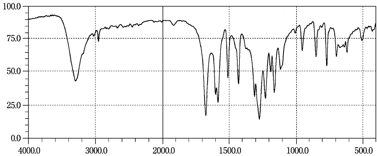
Methyl Parahydroxybenzoate
