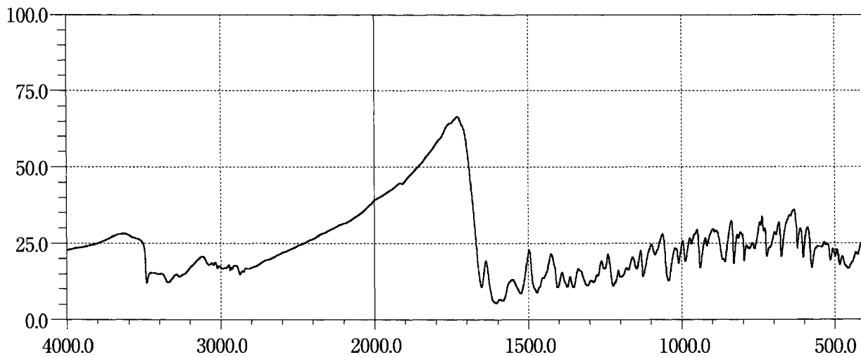
Minocycline Hydrochloride
