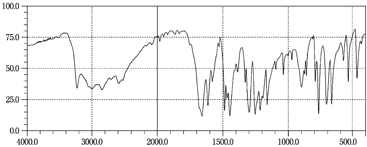
Salicylic Acid
