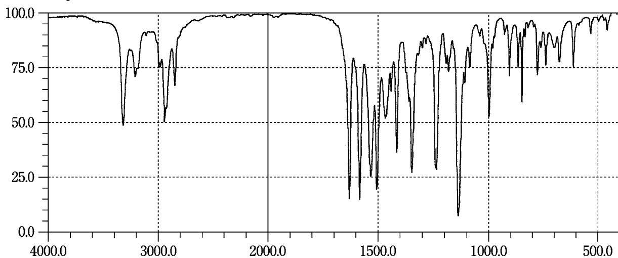
Troxipide
