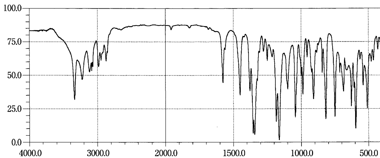
Mefruside
