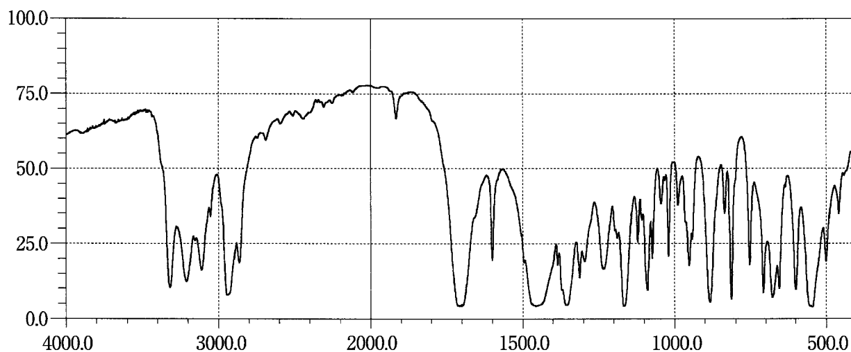
Tolazamide
