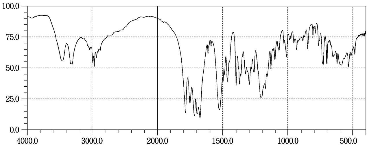
Piperacillin Hydrate
