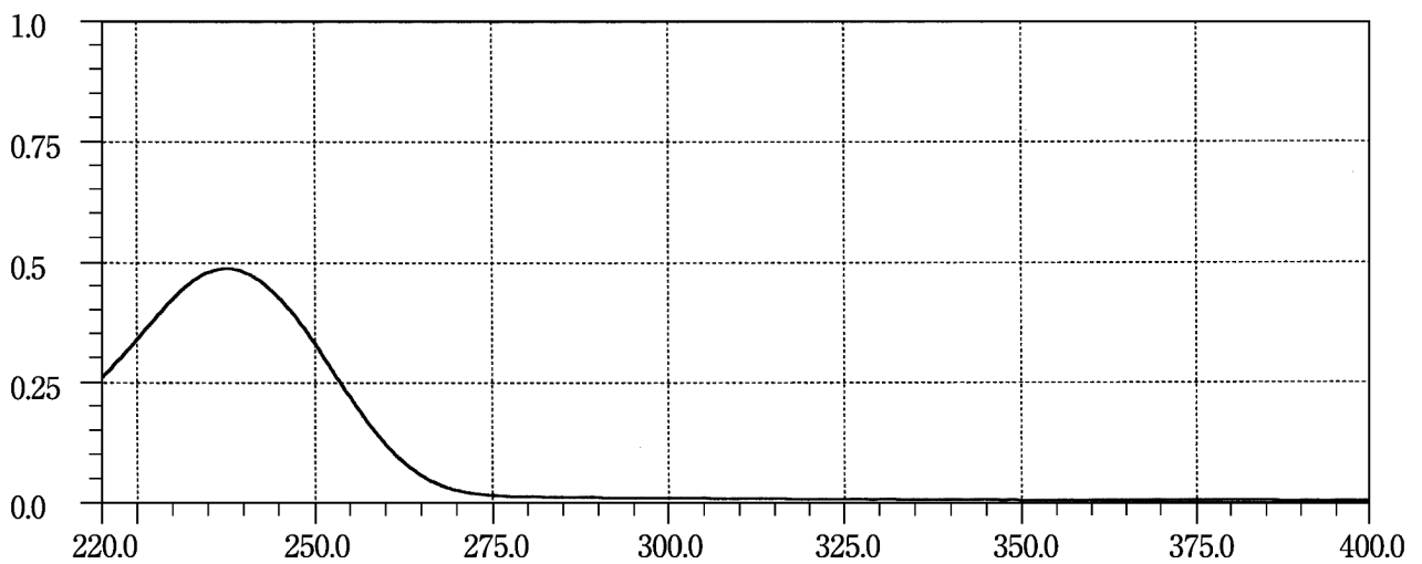
Spirolactone
