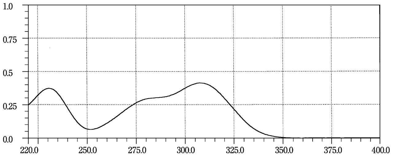
Oxybuprocaine Hydrochloride
