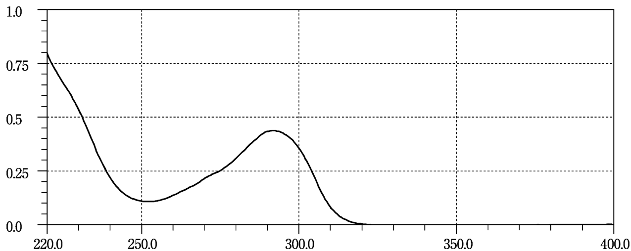
Rabeprazole Sodium
