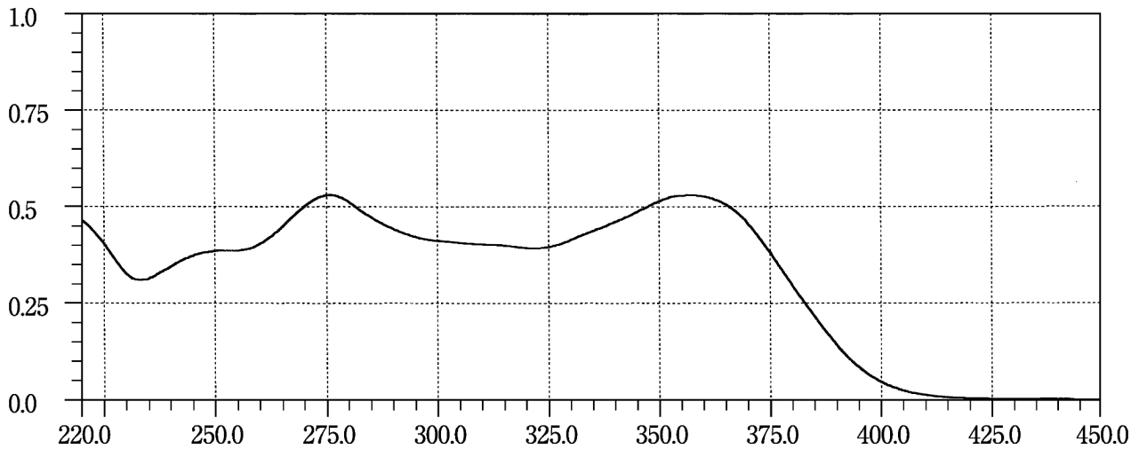
Tetracycline Hydrochloride
