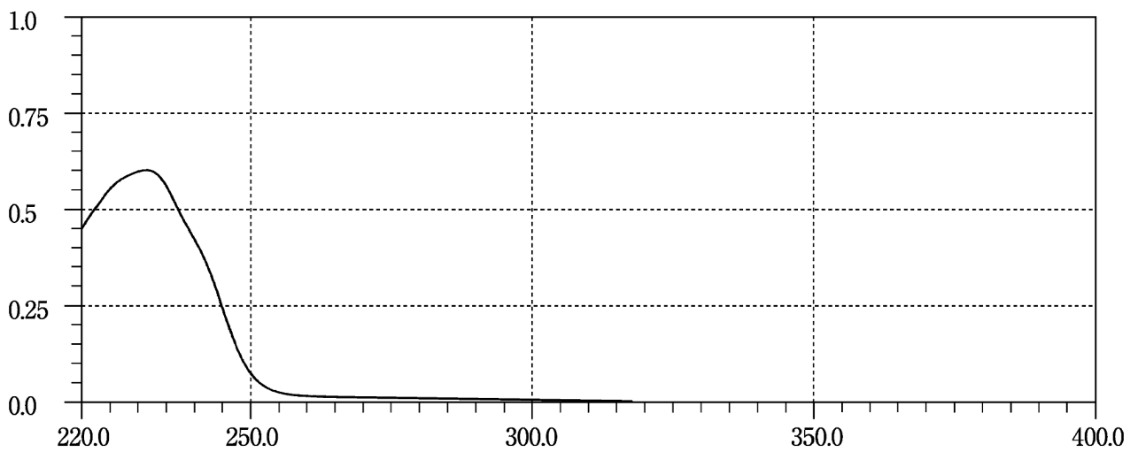
Spiramycin Acetate
