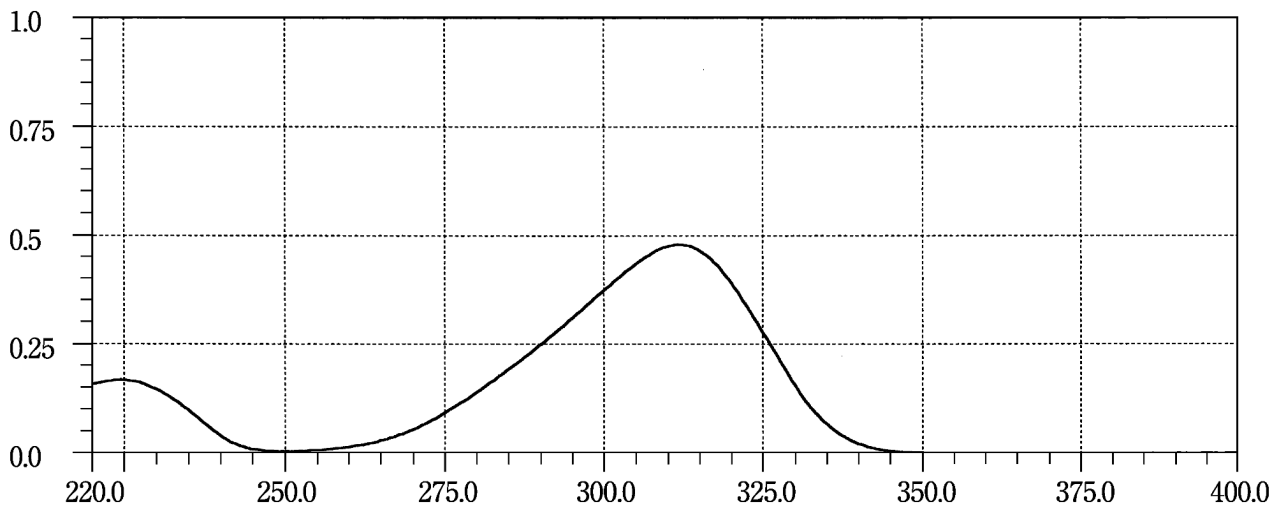
Tetracaine Hydrochloride
