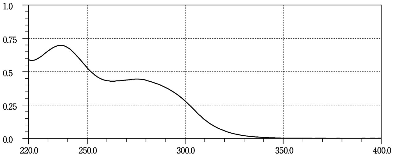
Tamoxifen Citrate
