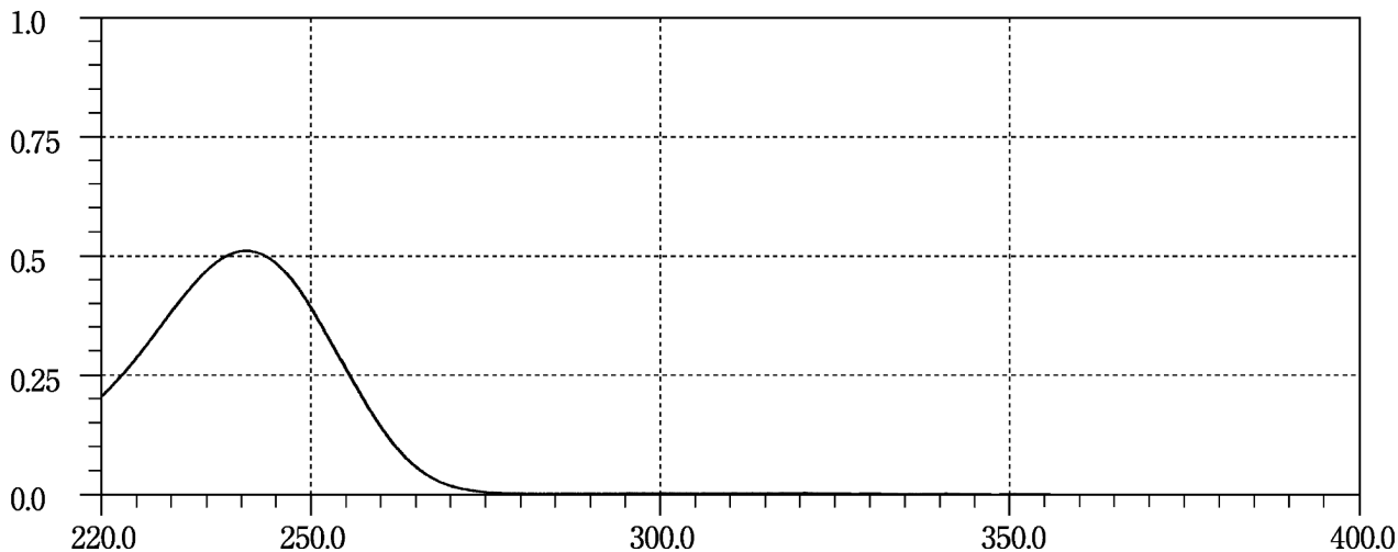
Testosterone Propionate
