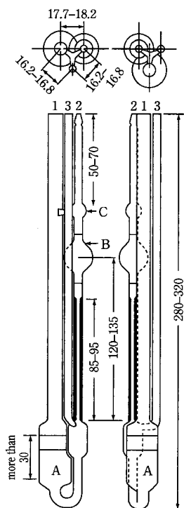
Fig. 2.53-1 Capillary tube viscometer
