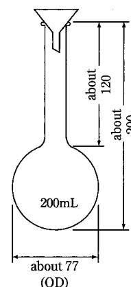
Fig. 1.13-1 Hydroxyl value determination flask
