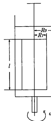
Fig. 2.53-2a Coaxial double cylinder-type rotational viscometer
