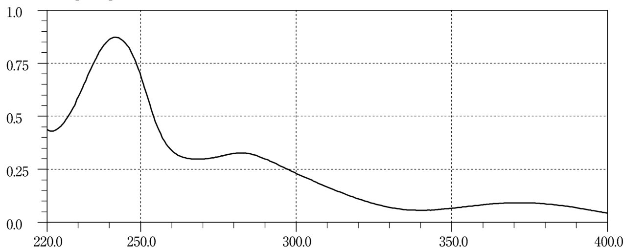
Flutoprazepam
