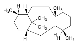
taxane
