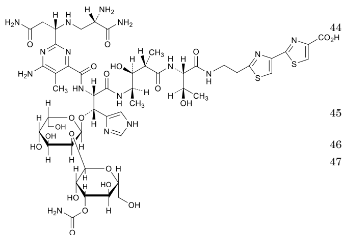
38 bleomycinic acid
