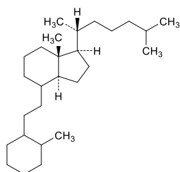
33 9,10-secocholestane
